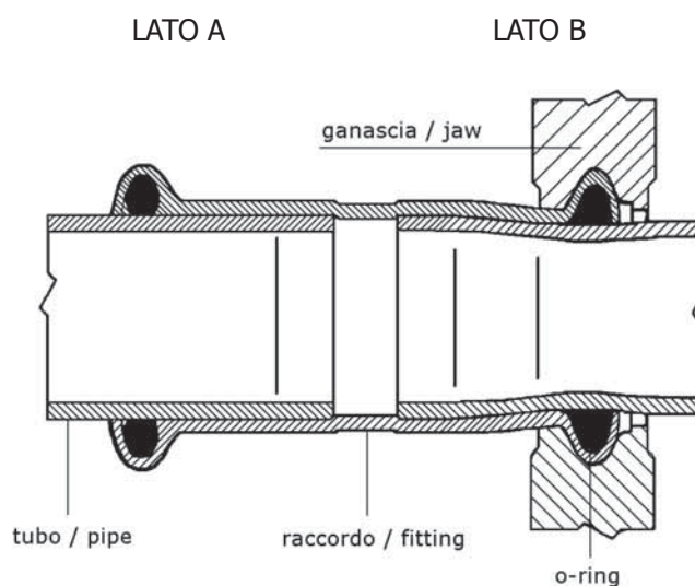
Fig. 1: Pipe and fitting:
